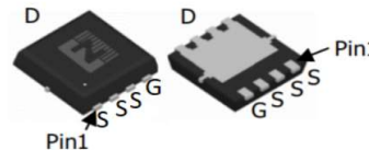
DFN3*3
